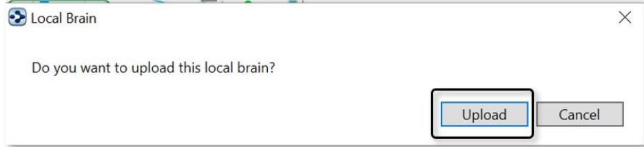
Figure 257. Confirming Upload
