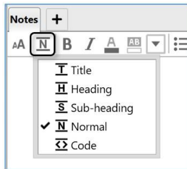
Figure 185. Paragraph Styles
