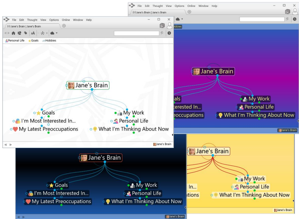
Figure 62. Sample Themes
