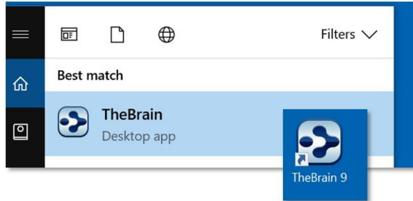
Figure 15. Starting TheBrain
