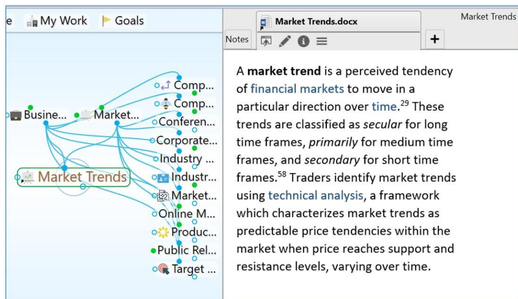
Figure 205. Content Preview
