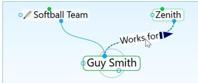
Figure 158. One-Way Link
