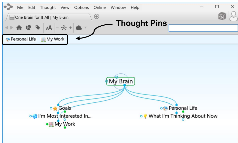
Figure 46. Pins
