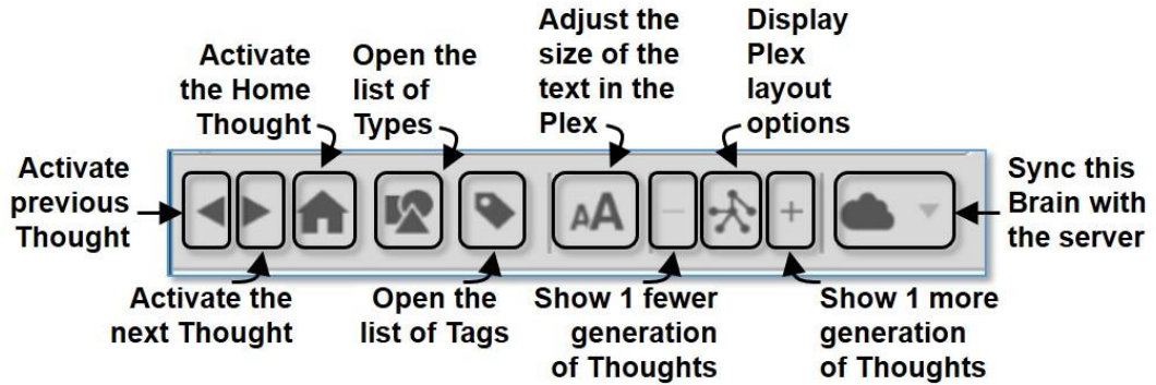
Figure 20. TheBrain Toolbar
