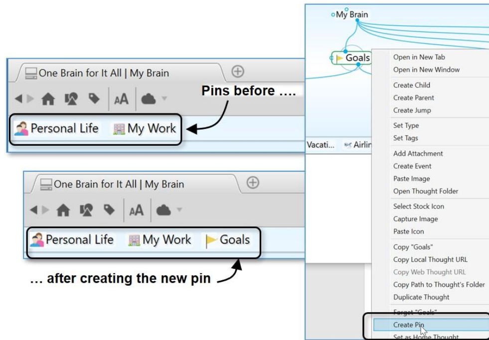
Figure 47. Creating Pins
