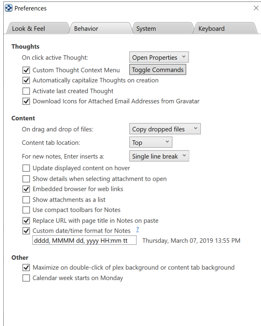
Figure 82. Behavior Preferences
