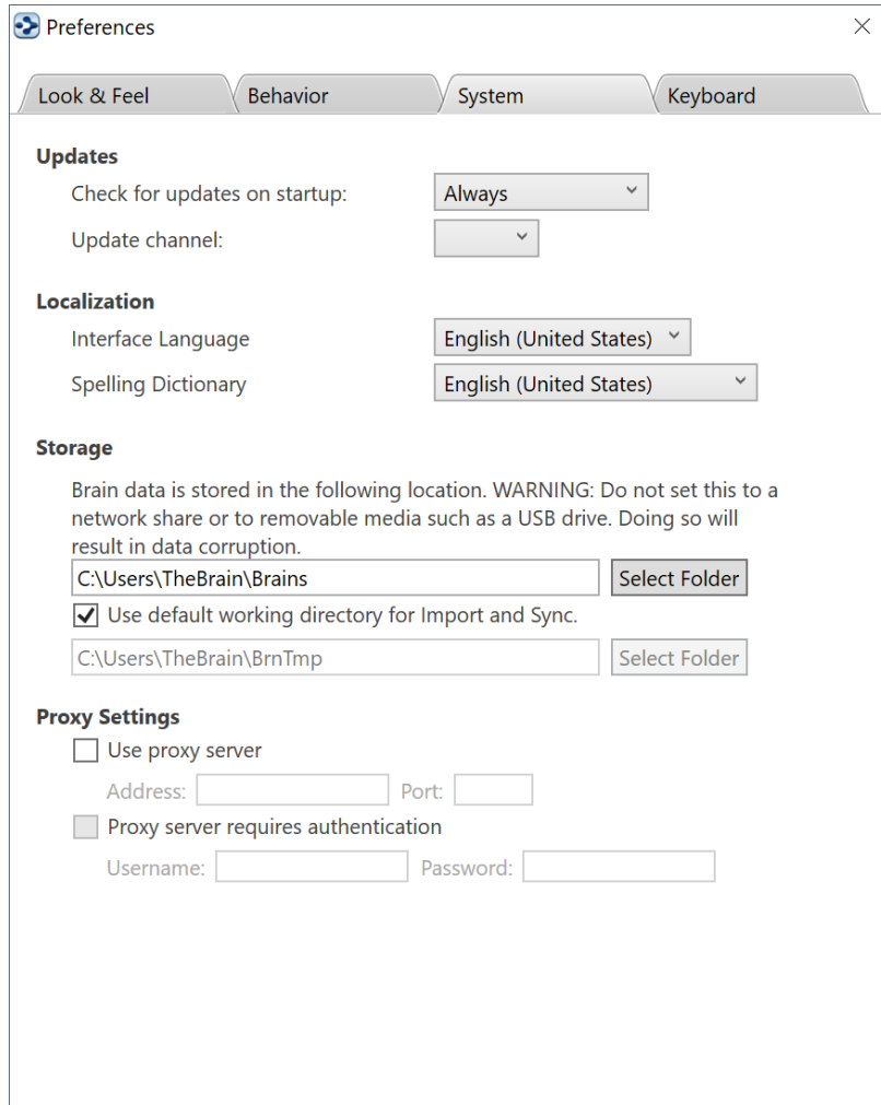
Figure 83. System Preferences
