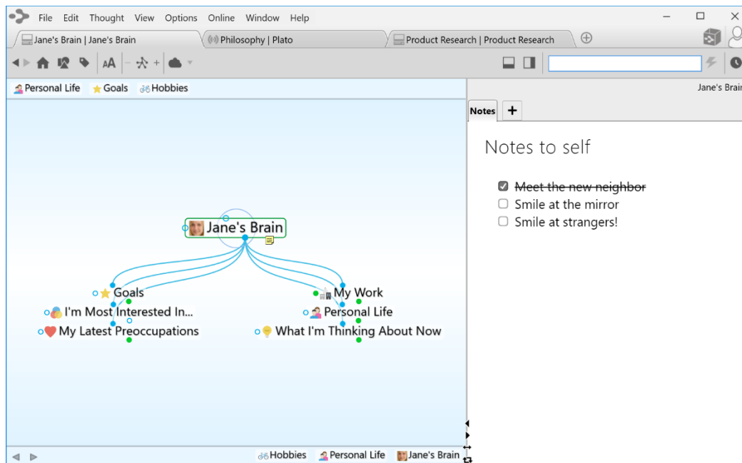
Figure 1. TheBrain Interface
