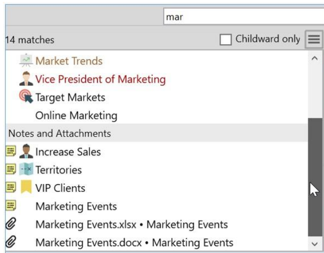
Figure 53. Search Results
