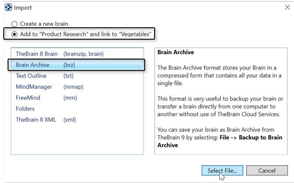
Figure 265. Merging Brains
