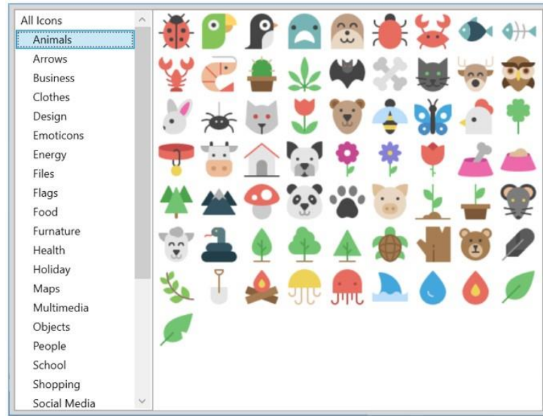
Figure 121. Icon Choices
