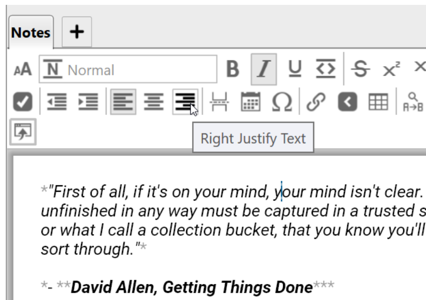
Figure 192. Paragraph Alignment
