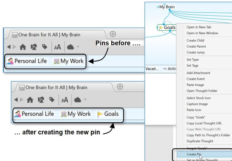
Figure 48. Creating Pins
