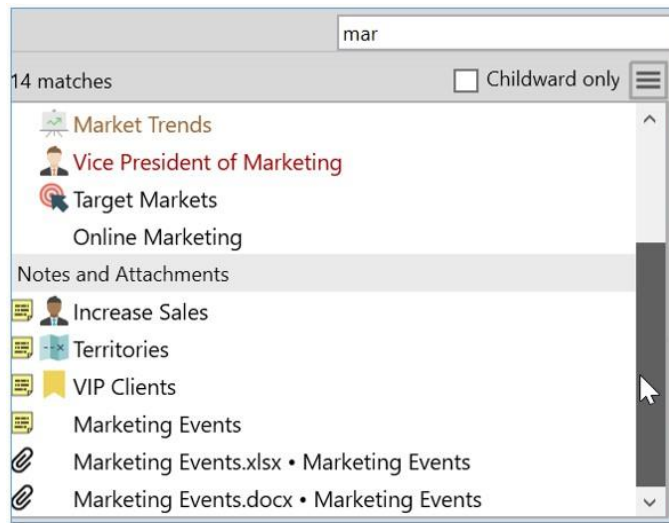
Figure 54. Search Results
