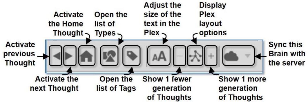
Figure 20. TheBrain Toolbar
