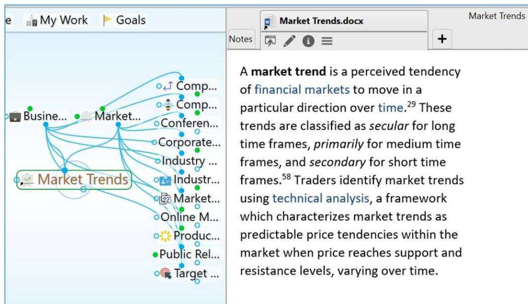
Figure 214. Content Preview
