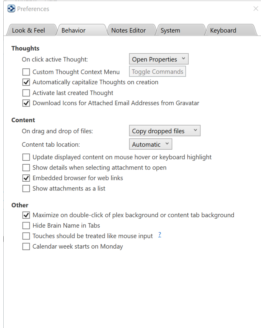
Figure 83. Behavior Preferences
