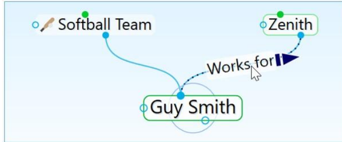
Figure 162. One-Way Link
