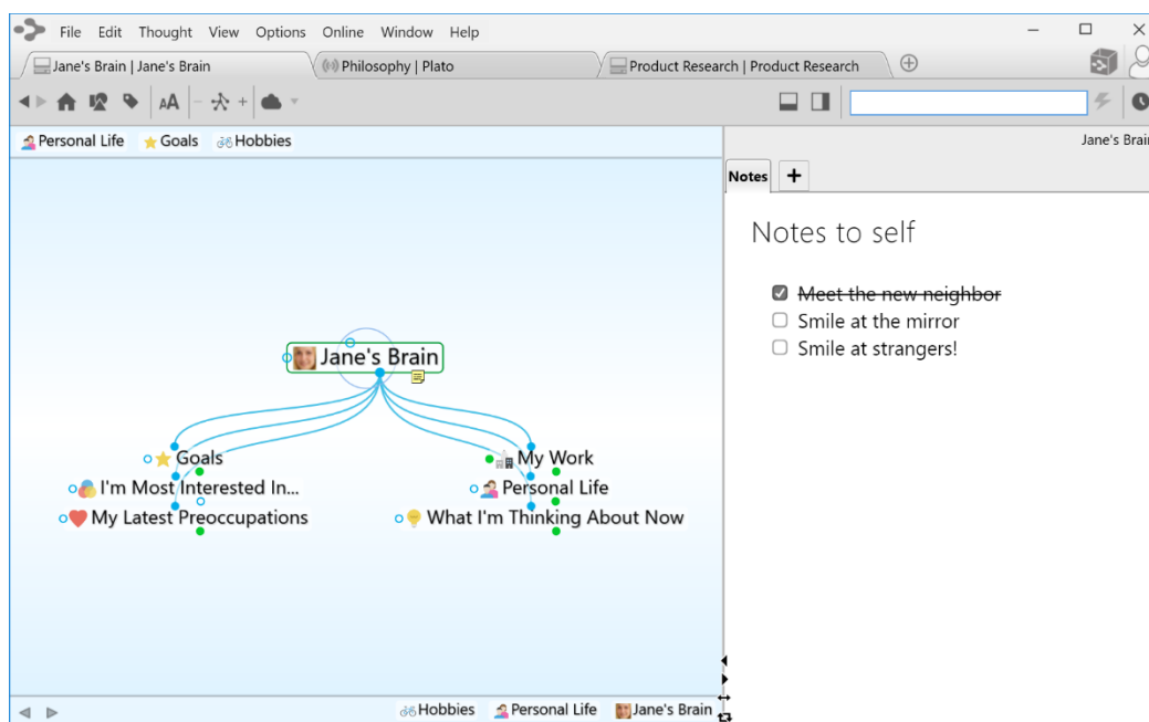
Figure 1. TheBrain Interface
