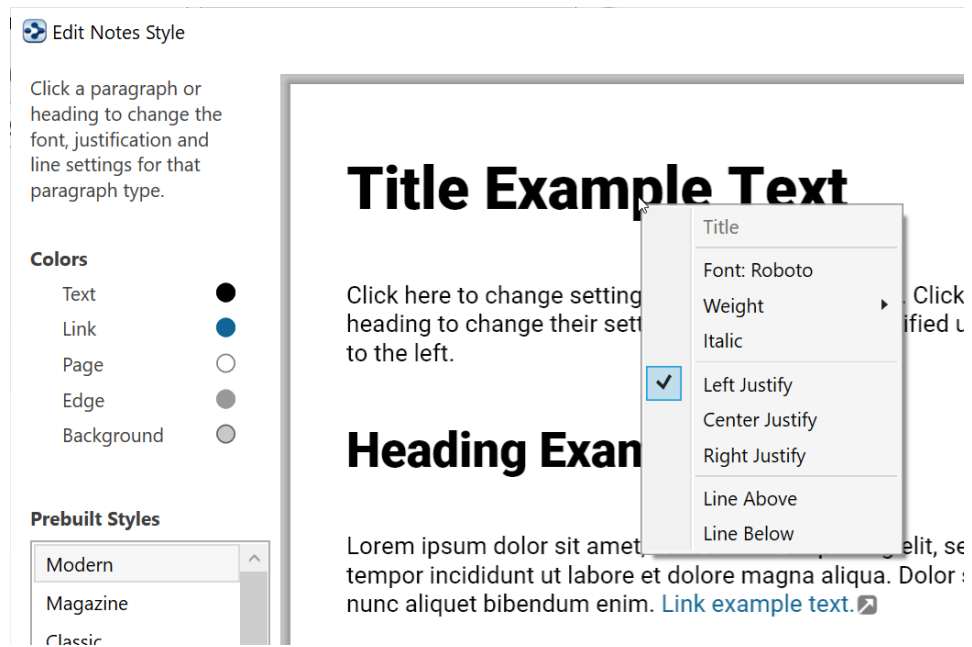
Figure 190. Paragraph Styles
