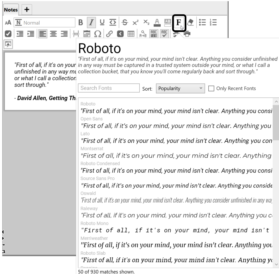
Figure 193. Fonts
