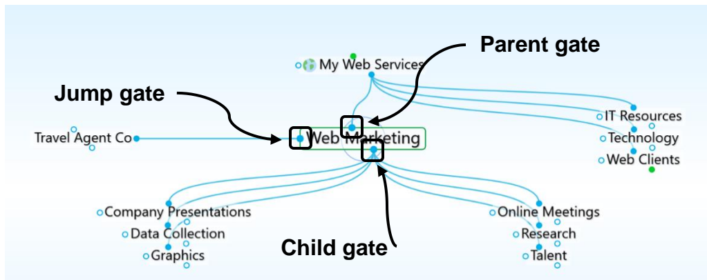
Figure 7. Thought Gates
