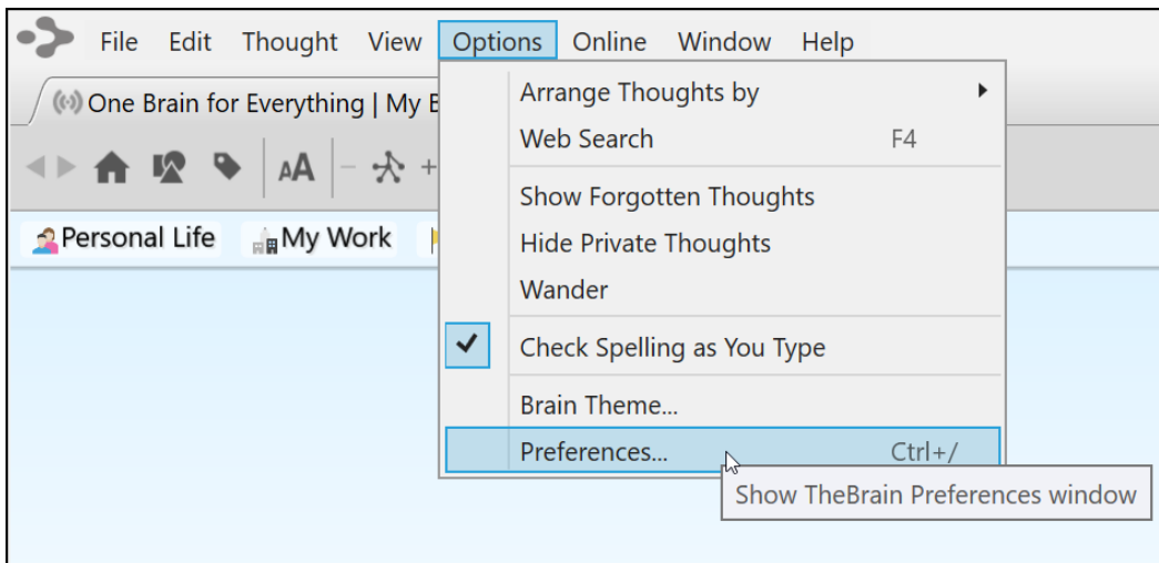
Figure 81. Accessing Preferences
