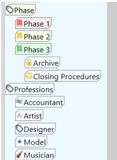
Figure 151. Nested Tags
