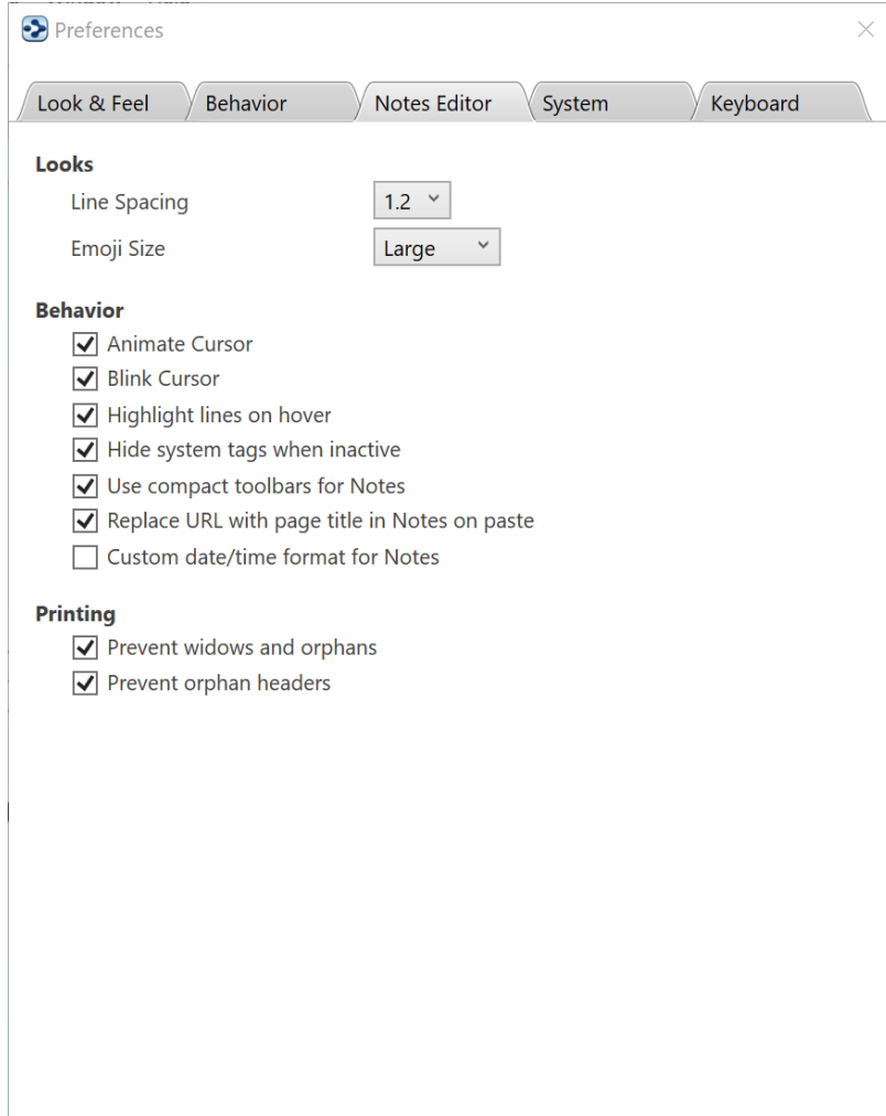
Figure 84. System Preferences
